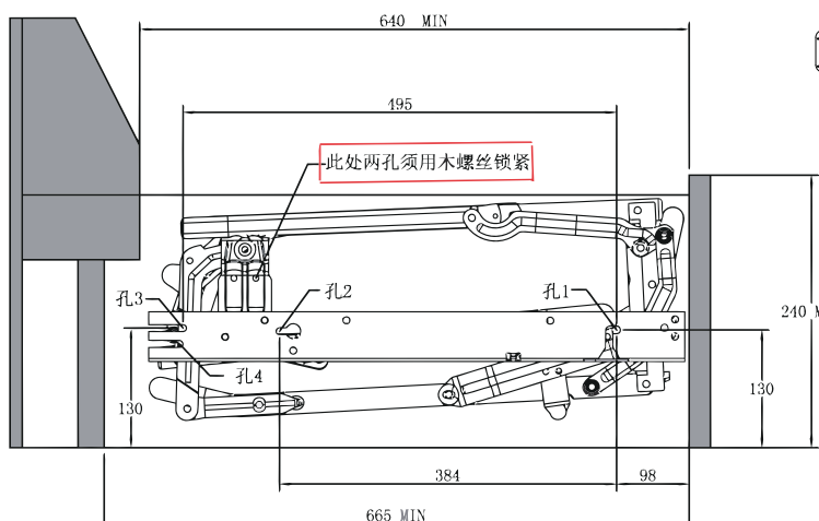
M6 Mounting Drawing
