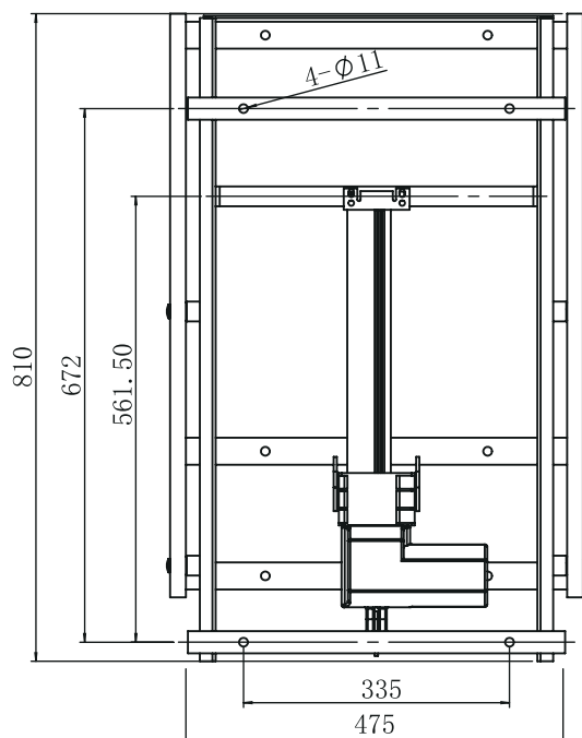
Base Frame Dimensions
